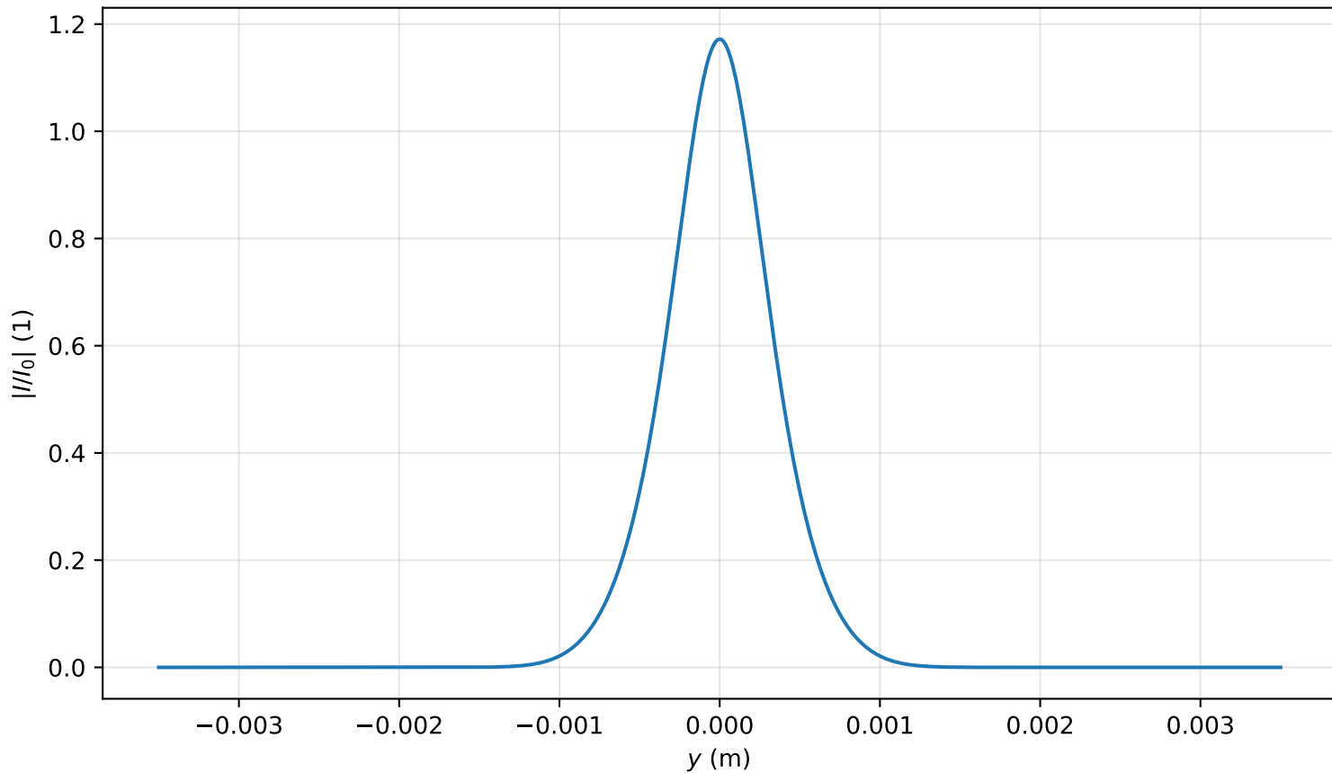
Intensity profile I(x=0, y, z=0.637)/I_0 , P_{in}=0.8P_{cr} , artificial time
